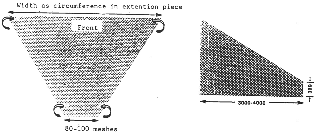
Figure 5. Cutting and construction of guiding funnel
