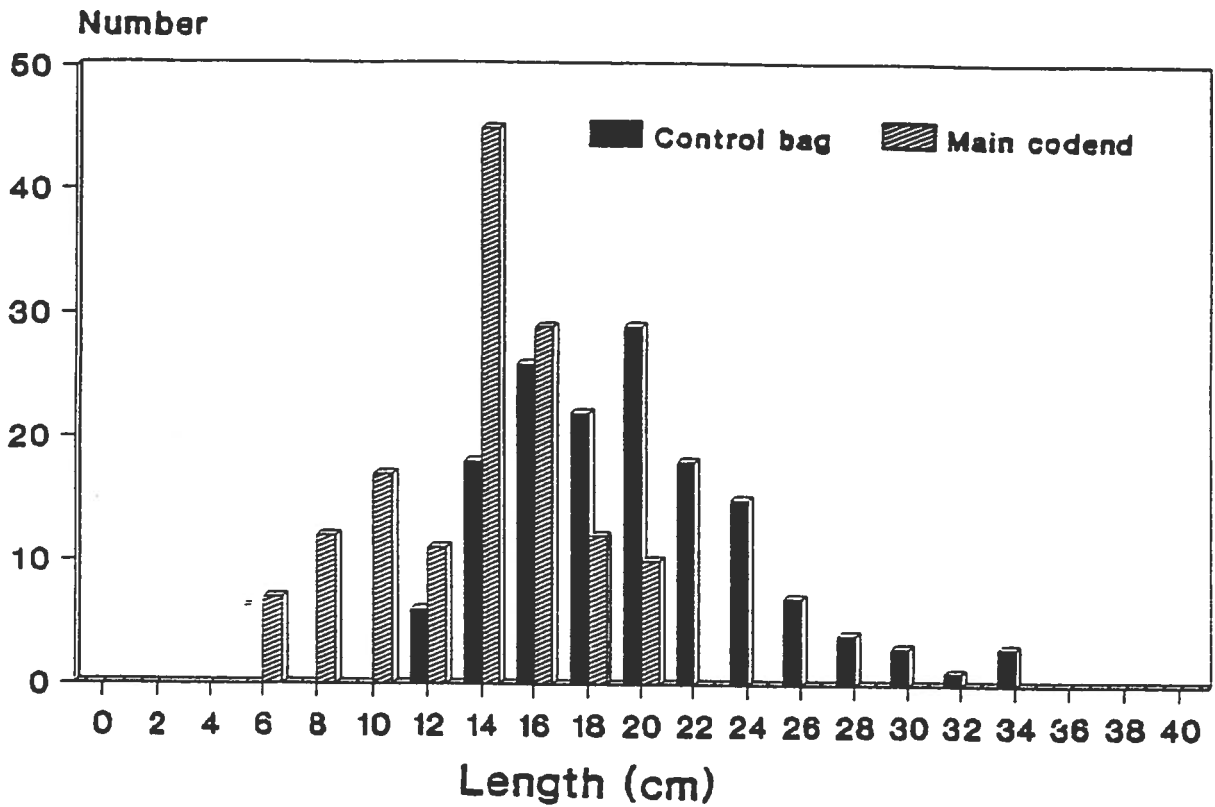
Figure 14. Length distribution of long rough dab in the main codend and the control bag.
