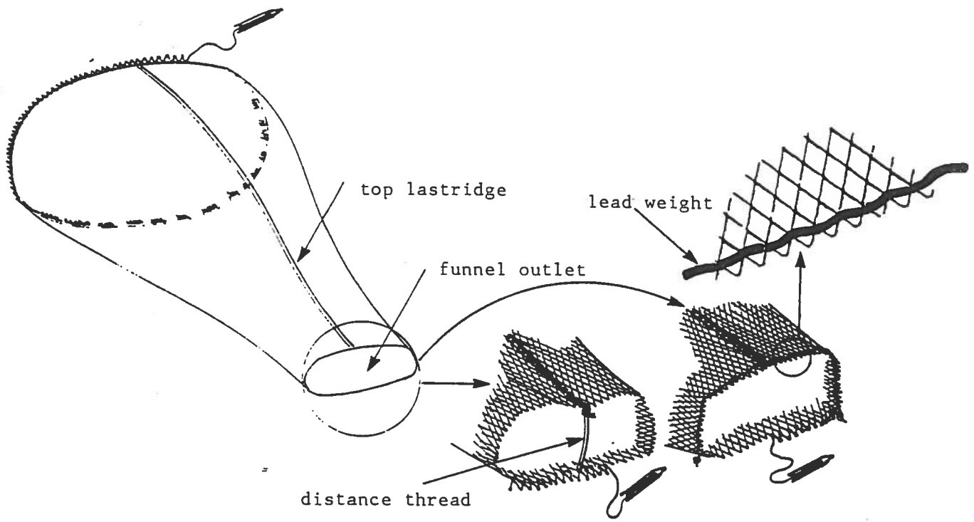
Figure 6. Illustration of guiding funnel
